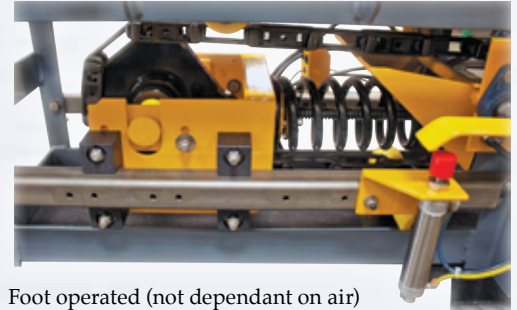
Foot operated (not dependant on air) manual roller call-up with lock.
