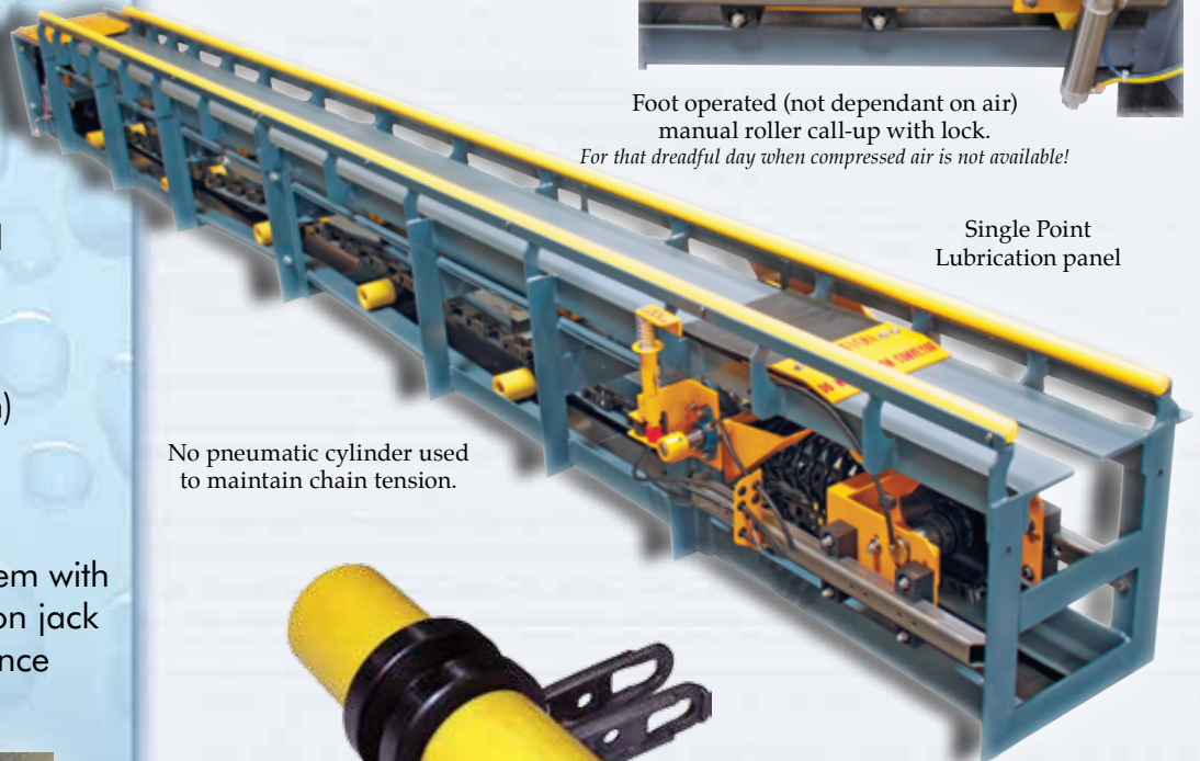
X458 Chain. Self-locking drop forged, the strongest and longest lasting chain in the industry
